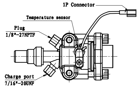
UWX550-5200 Hose Manifold / Shut-off Valve Detail
