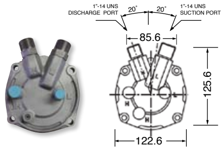
Part no 21503-000360 Vertical type
