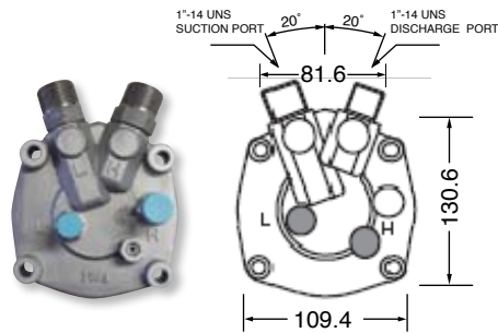
Part no 21503-000350 Vertical type
