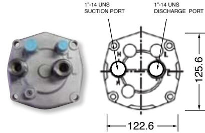
Part no 21504-000140 Horizontal type
