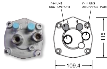
Part no 21504-000130 Horizontal type
